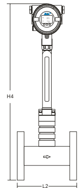
Flange Type
